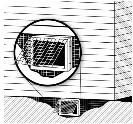
Figure 3. A one-way door constructed to allow an animal to exit but not to return. Screen door must overlap frame to prevent re-entry.
